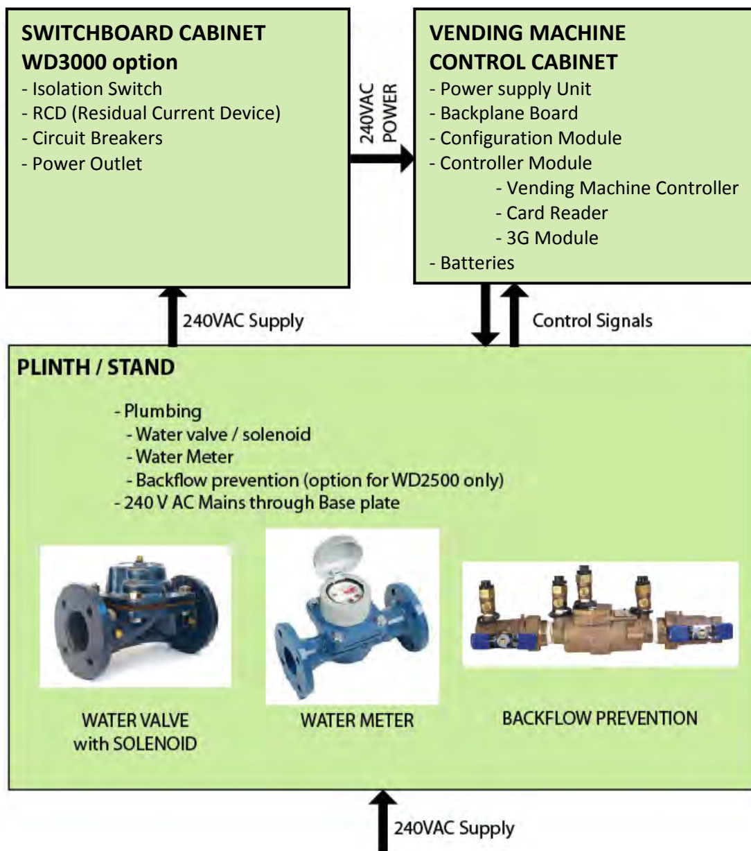
Figure 5 - Machine Breakdown
