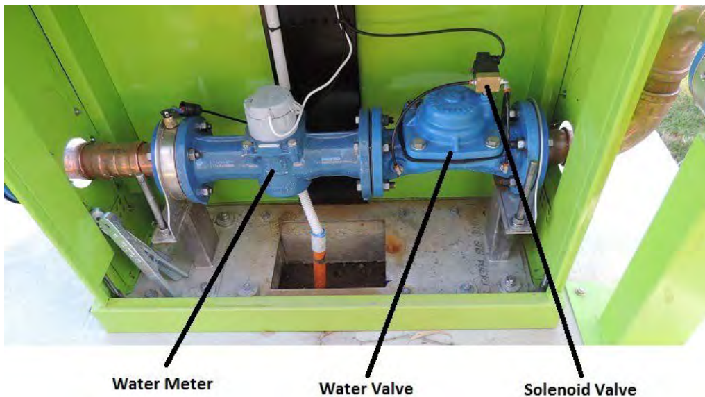
Figure 9 - WD3000 Plumbing
