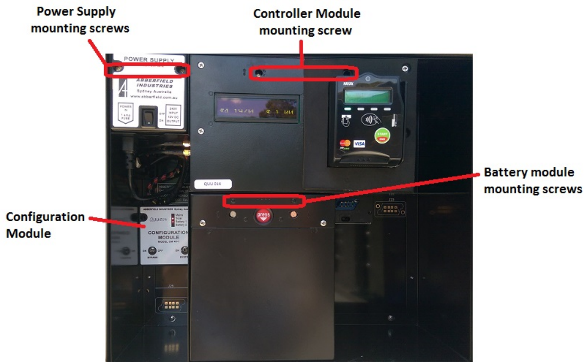
Figure 7 - Module mounting screws
