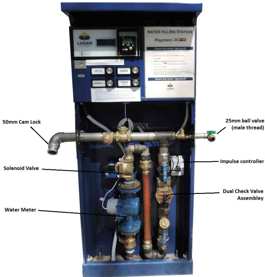
Figure 8 - WD2500 with internal backflow prevention
