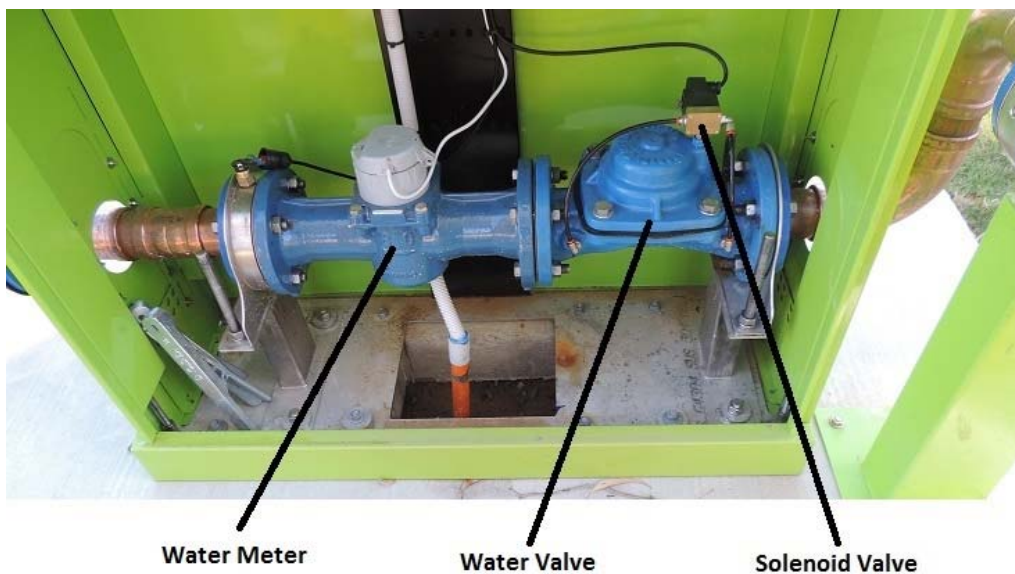
Figure 9 - WD3000N Plumbing
