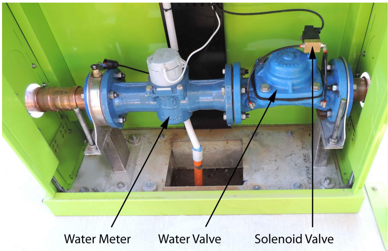
WD3000N Plumbing
